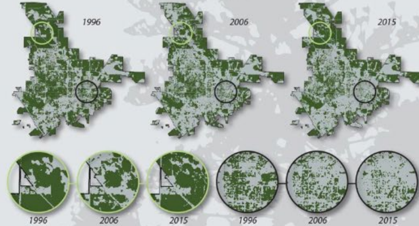
Changes to Gainesville's canopy occurred between 1996 and 2015. In some areas (left), canopy was lost then gained, likely due to timber harvest followed by reforestation. In other areas of the city (right), canopy has been lost over time without gains.
