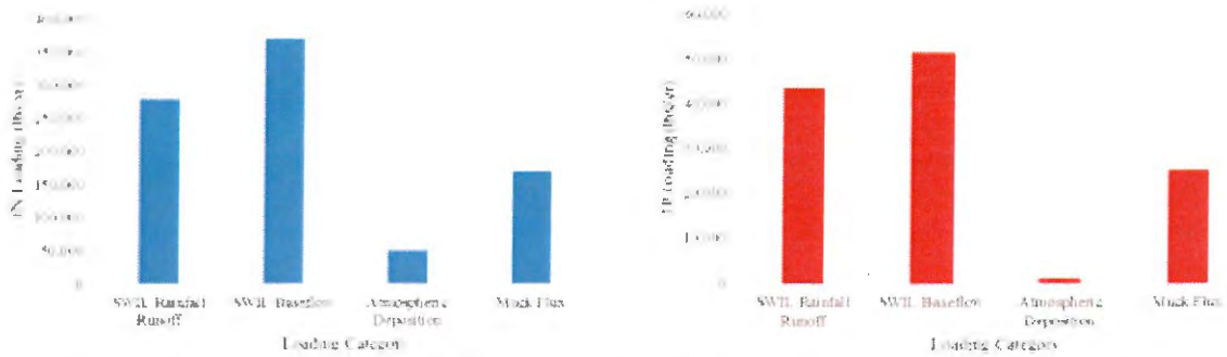
Figure 5: Central IRL TN (left) and TP (right) Annual Average Loads by Source
