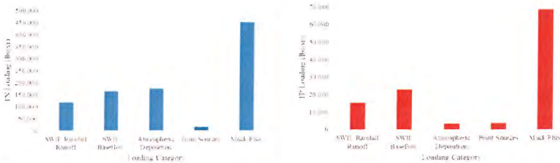
Figure 3: Banana River Lagoon TN (left) and TP (right) Annual Average Loads by Source
