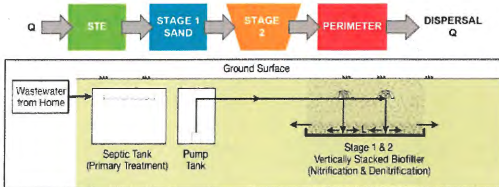
Figure 10: Example Diagram of an In-Ground Stacked Biofilter
